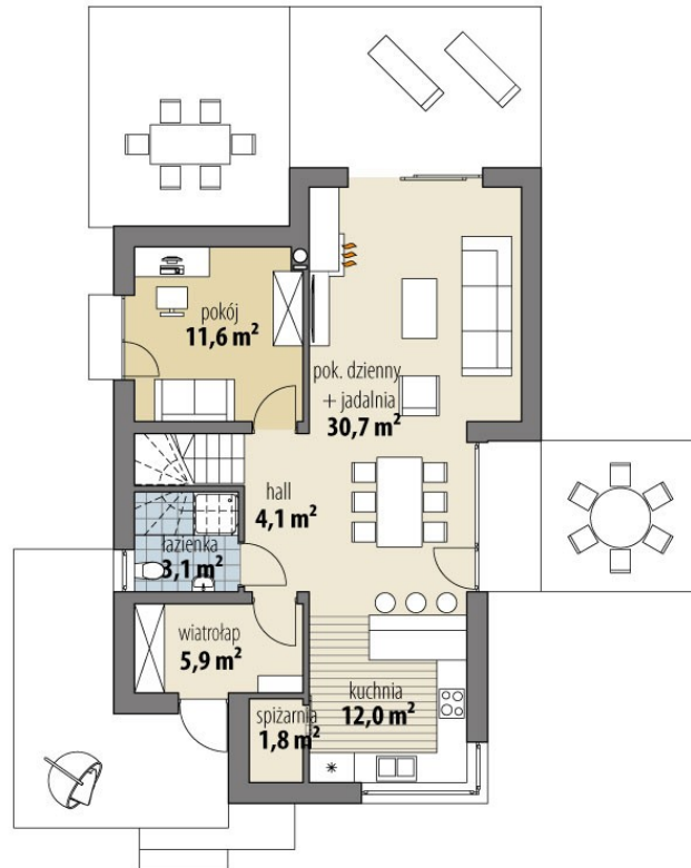
PARTER
