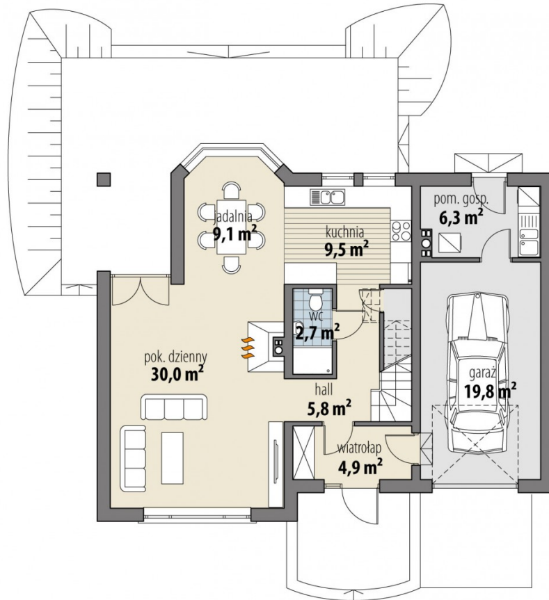
PARTER
