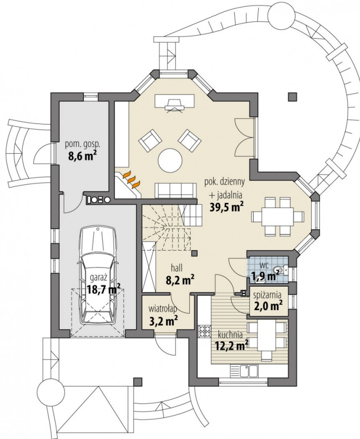
PARTER
