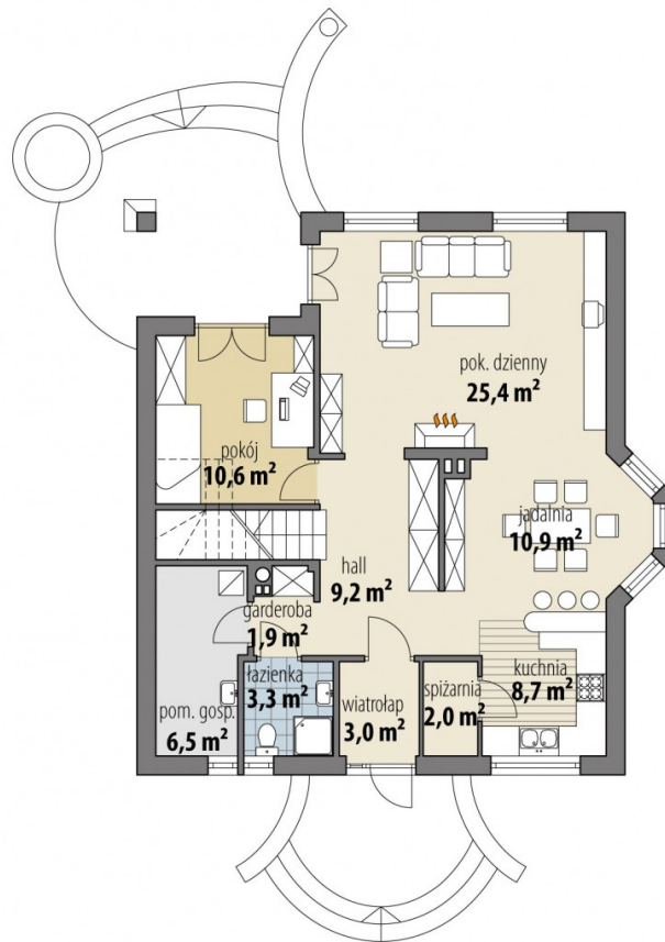
PARTER
