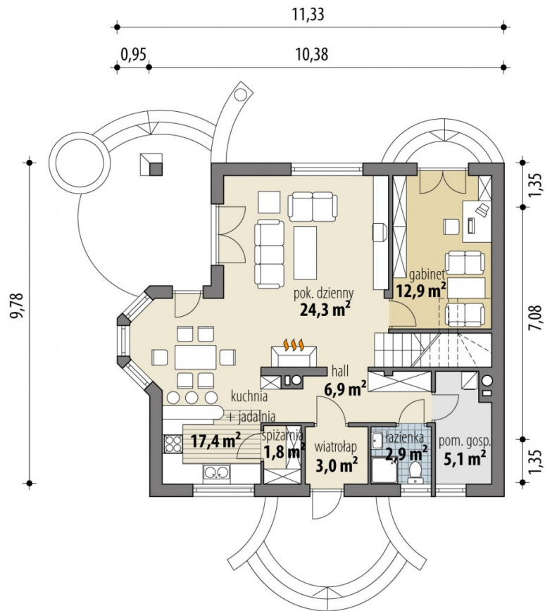
PARTER
