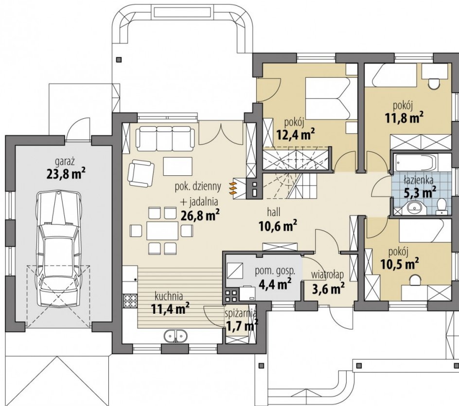
PARTER
