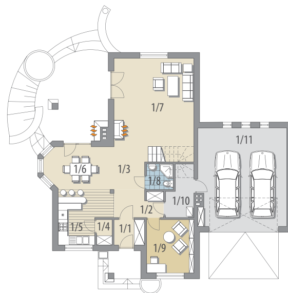
Parter
