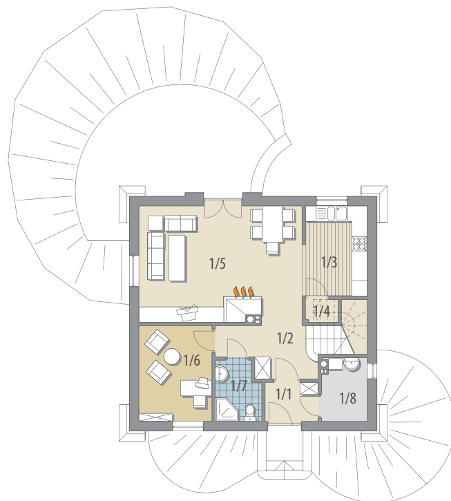
Parter
