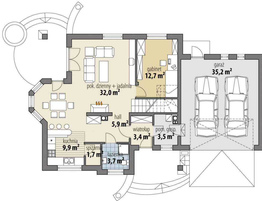
PARTER
