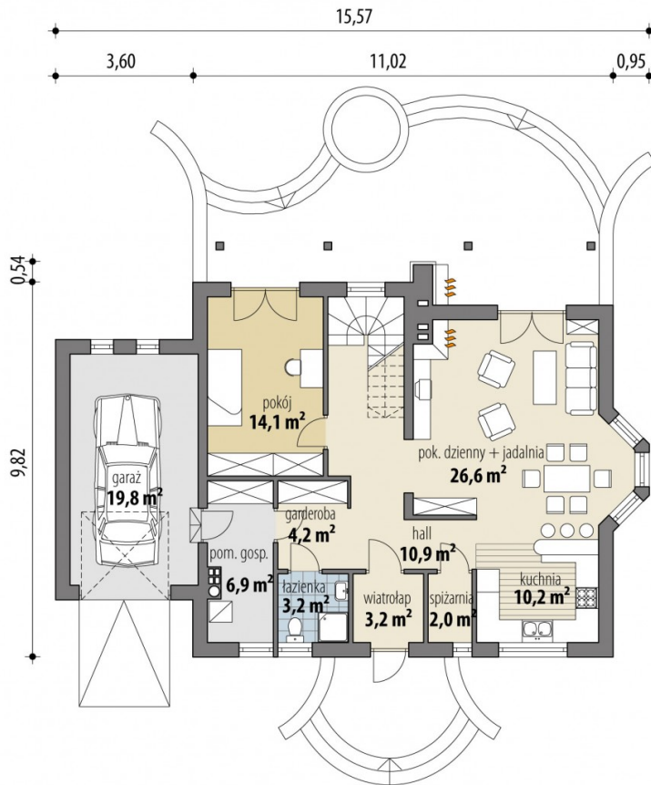
PARTER
